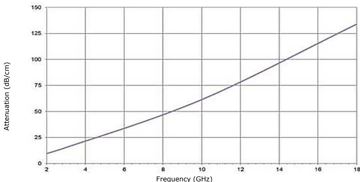
Typical attenuation AHF-STB-PP-220
