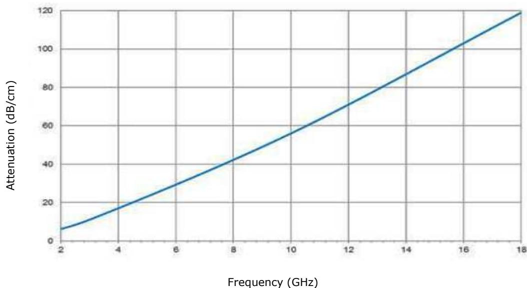
Typical attenuation AHF-HLE
