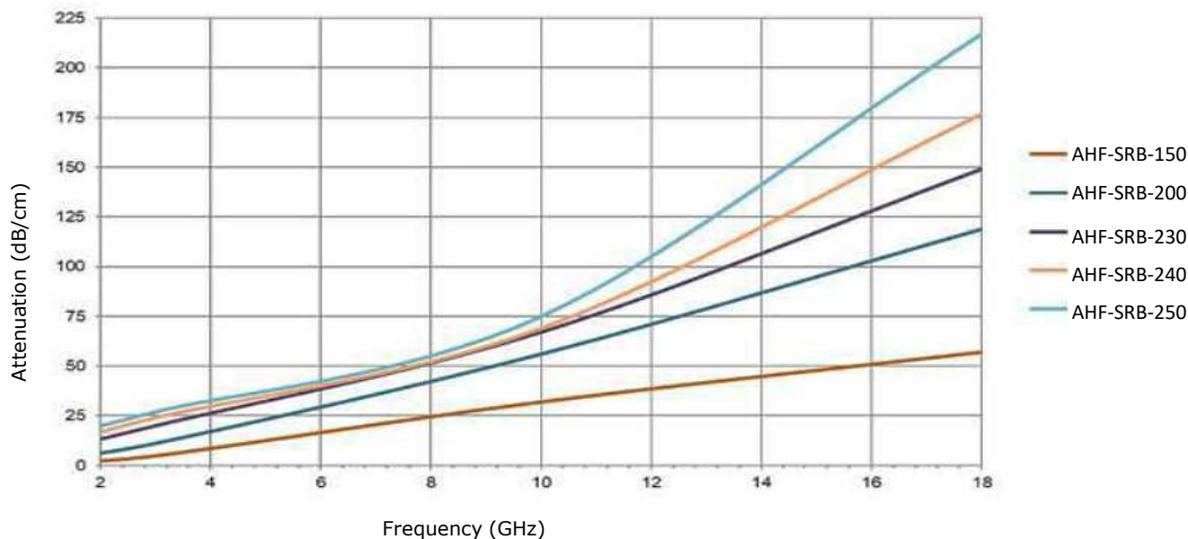
Typical attenuation AHF-SRB
