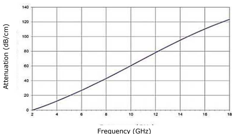
Typical attenuation AHF-MLE
