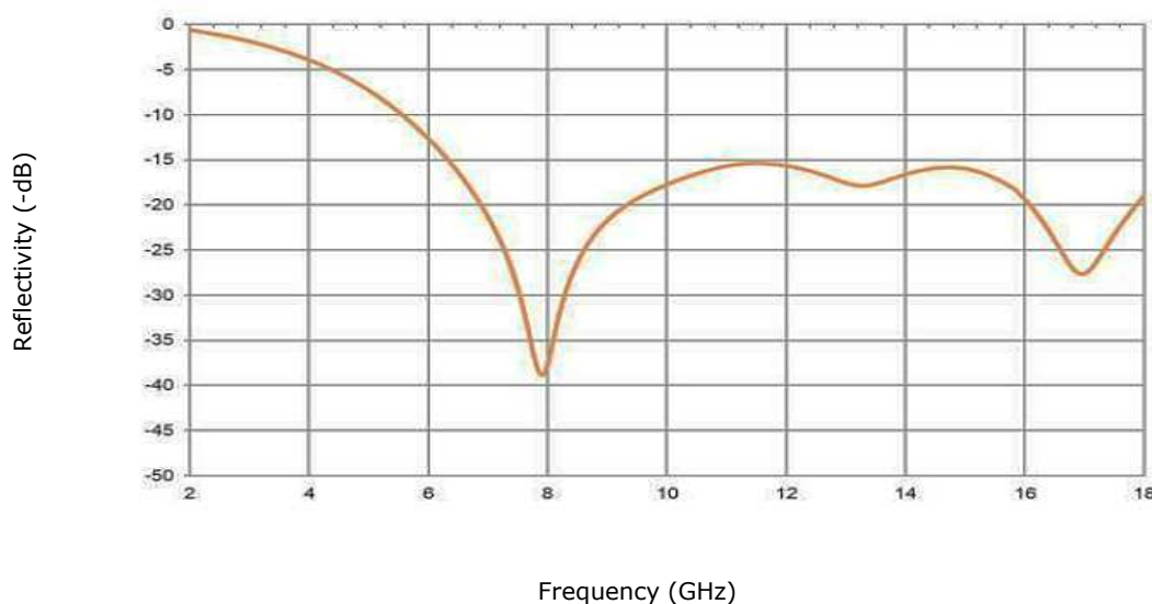
Typical reflectivity AHF-NSA
